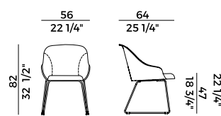
918/SLI sedia base slitta \ sled base chair
