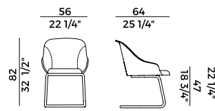
918/UI sedia base cantilever \ cantilever base chair
