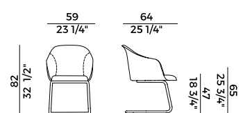
918/PUI poltroncina base cantilever \ cantilever base armchair
