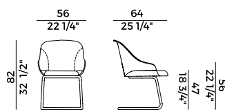
918/U sedia base cantilever \ cantilever base chair
