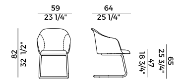
918/PUI poltroncina base cantilever \ cantilever base armchair
