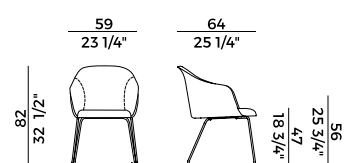
918/PSLI poltroncina base slitta \ sled base armchair
