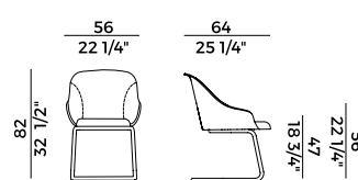
918/UI sedia base cantilever \ cantilever base chair
