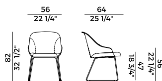
918/SL sedia base slitta \ sled base chair
